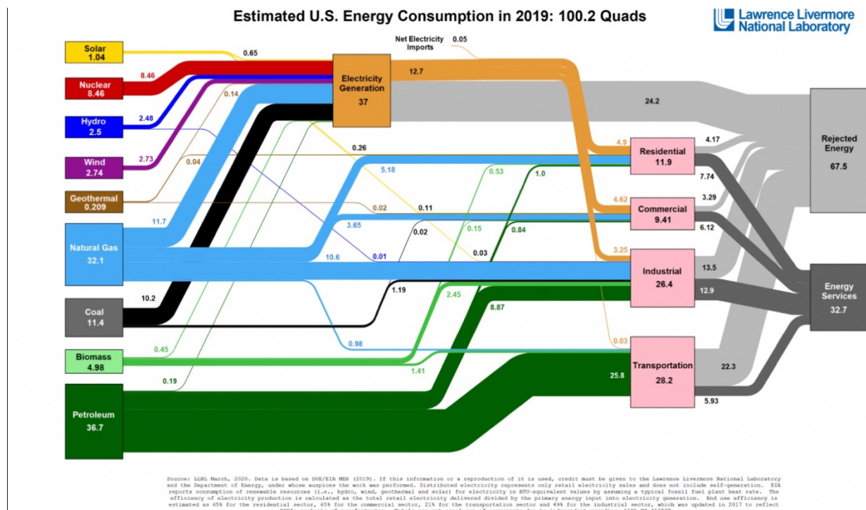
Figure A-1. U.S. Energy System Structure and Losses (LLNL, 2019)
